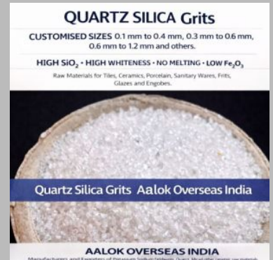
Quartz Grains
