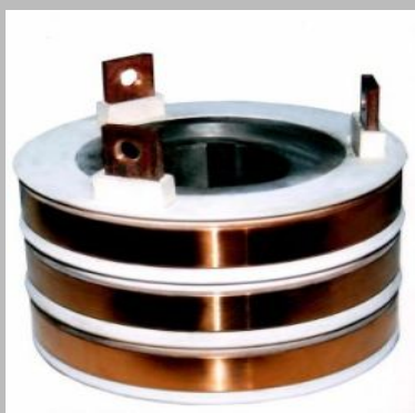
Slip Ring For GEC Motor
