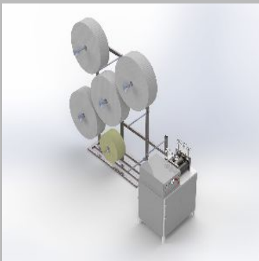
Automatic Sanitary Napkin Making Machine
