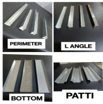
GI Ceiling Channel L Angle
