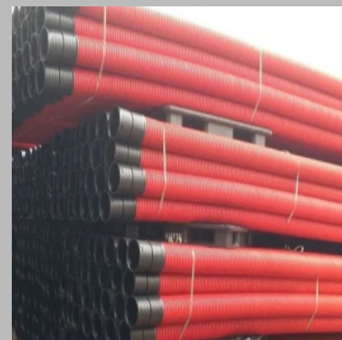
OD 75 & ID 61 mm Double Wall Corrugated Pipes
