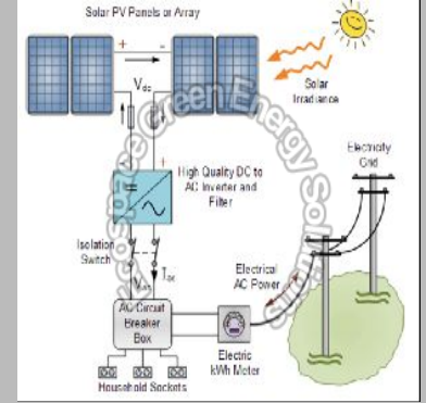
Solar On Grid System
