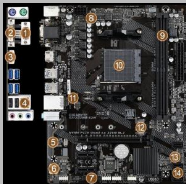
Gigabyte GA-A320M-S2H Motherboard
