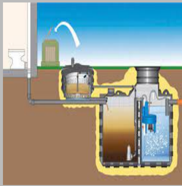
Domestic Sewage Treatment Plant
