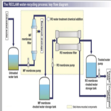
Industrial Water Treatment Plant
