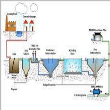
Water Treatment System
