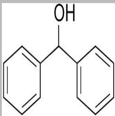
benzhydrol
