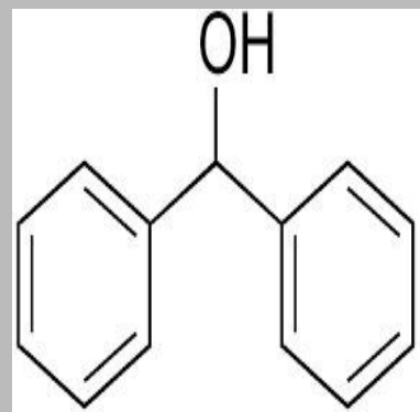
benzhydrol
