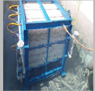
MBR Sewage Treatment Plant
