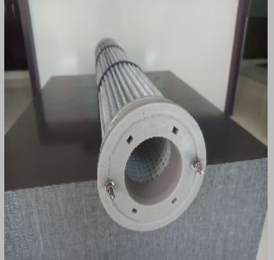
Bolted Type PU Molded Filter
