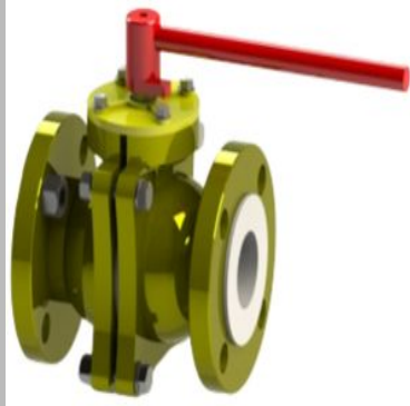
Lined Three Piece Ball Valve
