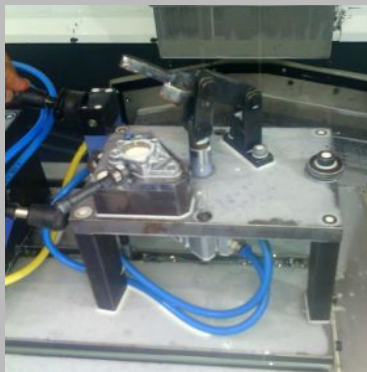
cnc machining fixtures
