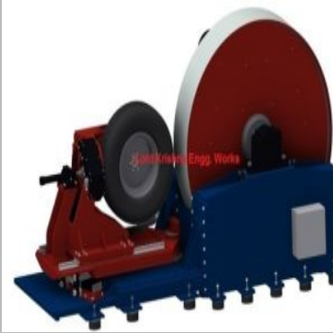
Tyre Endurance Test Rig
