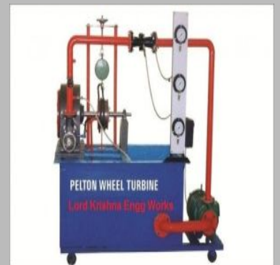
Pelton Turbine Test Rigs
