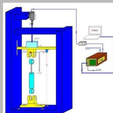
Shock Absorber Tester
