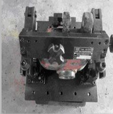
Manual Machining Fixtures
