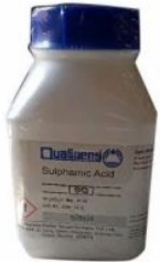
Sulfamic acid
