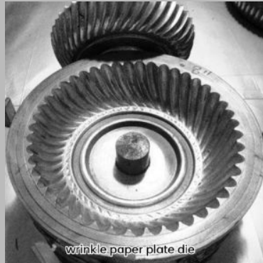
Diamond Paper Plate Die
