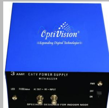
CATV Power Supply 3 AMP. - 60VAC
