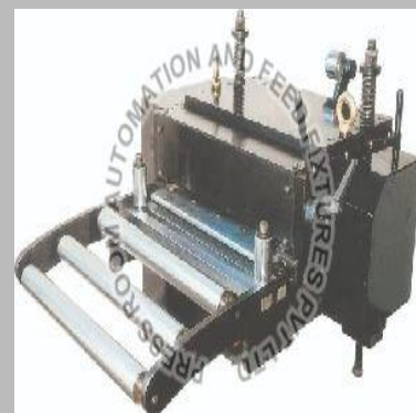
NC Servo Roll Feeder For Electrical Stamping
