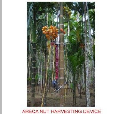
ARECA NUT HARVESTING DEVICE
