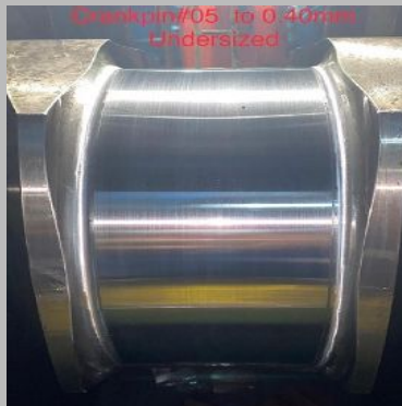
insitu machining of crankshaft repair services
