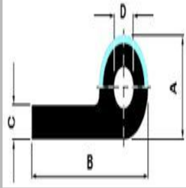
Hollow Dam Gate Bulb Seal
