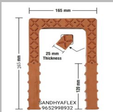
PVC Foot Rest
