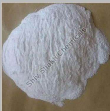
Sodium Chloride
