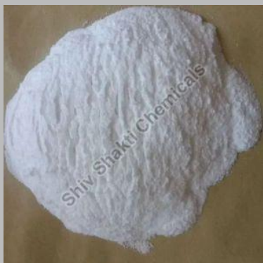
Sodium Chloride
