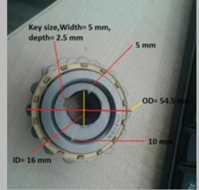
Cylindrical Bearing
