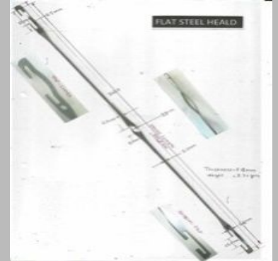
FLAT HEALD C TYPE & J TYPE
