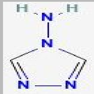
4 Amino 1 2 4-Triazole
