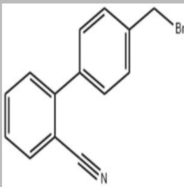
4' Bromomethyl 2 Cyanobiphenyl (Br.OTBN)
