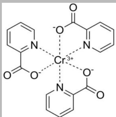
Chromium Picolinate
