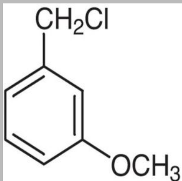
Methoxy Benzyl Chloride Chemical Intermediate
