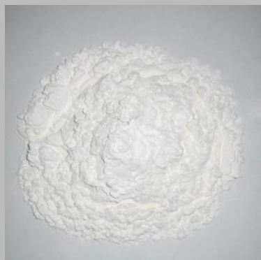
Industrial 4,4 Dimethoxy Triphenyl Methyl Chloride Intermediate
