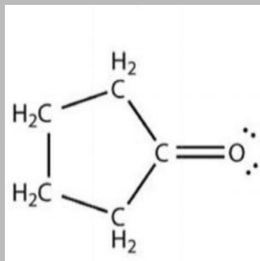
Cyclopentanone Chemical Intermediate
