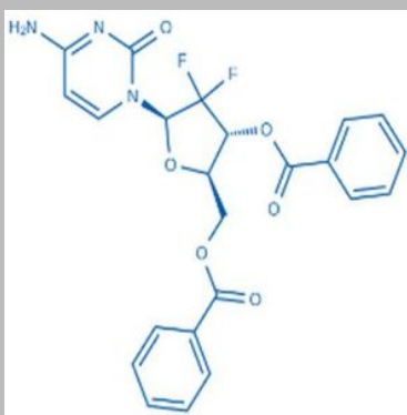
2,2 Difluoro-2-deoxycytidine-3-5-dibenzoate (T9)
