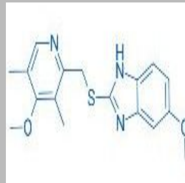
Omeprazole Sulphide
