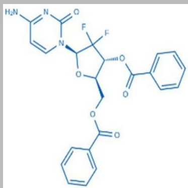
2,2 Difluoro-2-deoxycytidine-3-5-dibenzoate (T9)
