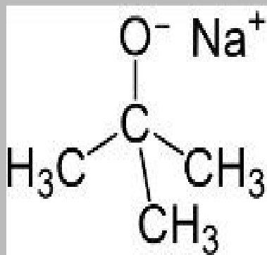
Sodium Tertiary Butoxide
