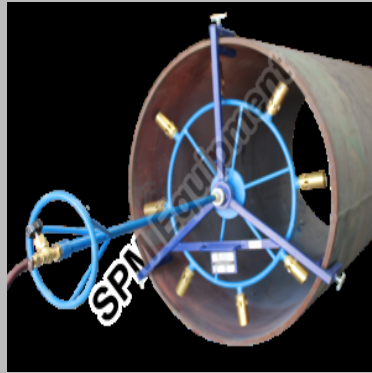
Internal Pipe End Heating Torch
