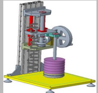
Manual Load Testing Jig
