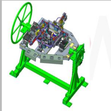
Rotary Welding Fixture
